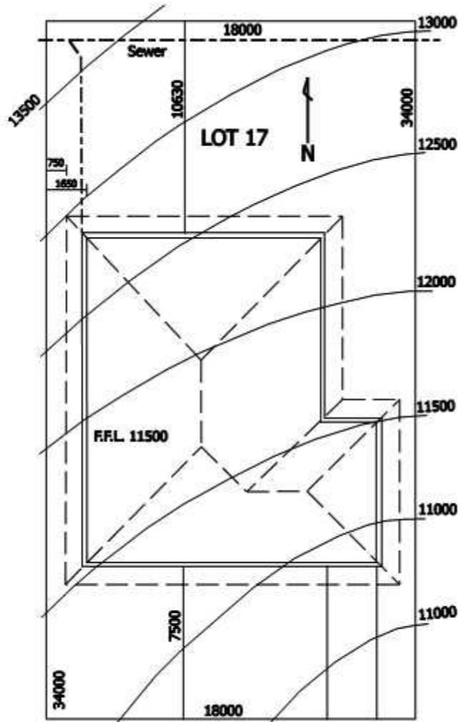
ROAD NAME Site Plan 1:200
