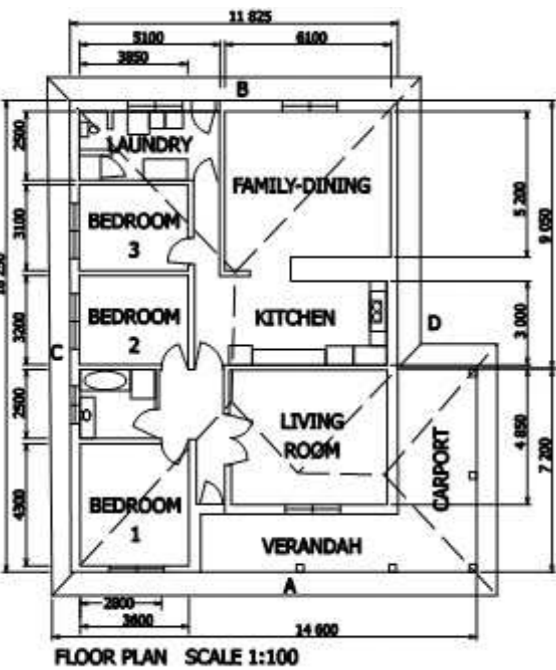
Typical Layout for a New Dwelling
