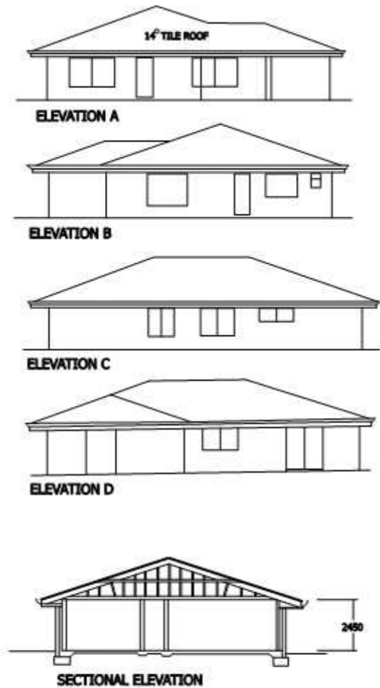
SECTIONAL ELEVATION
